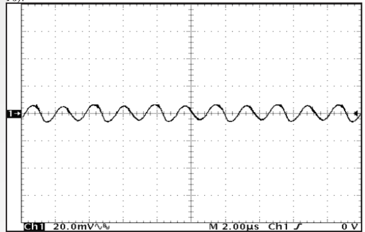
Figure 16: Output voltage ripple, V_{out} , at nominal input voltage and rated load current (20mV/div). Load capacitance: 1µ F ceramic capacitor and 10µF tantalum capacitor. Bandwidth: 10MHz. See Figure 14.
